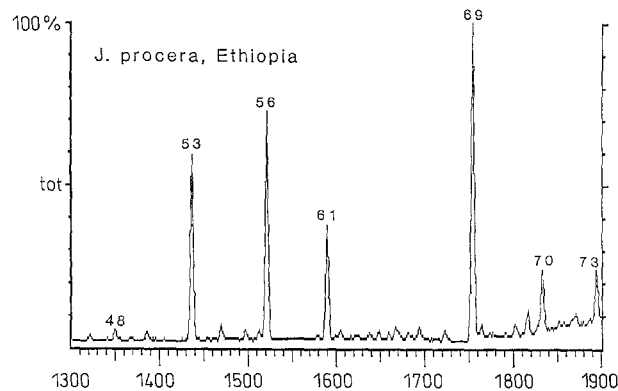
Fig. 4. Sesquiterpenes from the volatile leaf oils of J. excelsa , Greece, junipers at Abha, and J. procera , Ethiopia. The junipers from Abha are clearly J. procera . The peak numbers refer to Table 2, where complete analyses are reported
