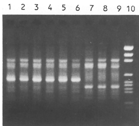
Fig. 2. RAPDs (primer 223) for juniper individuals. Lanes 1–3 J. procera , Ethiopia; lanes 4–6 junipers from Abha, Saudi Arabia; lanes 7–9 J. excelsa Greece; lane 10 molecular size markers. Note the 500 bp band uniting J. procera , Ethiopia and Abha and the 390-bp band characteristic of J. excelsa
