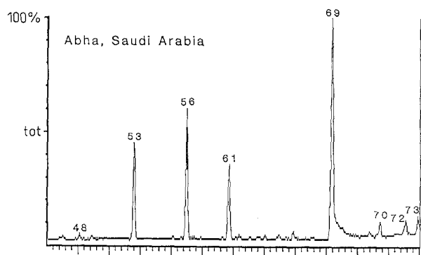
Fig. 2. RAPDs (primer 223) for juniper individuals. Lanes 1–3 J. procera , Ethiopia; lanes 4–6 junipers from Abha, Saudi Arabia; lanes 7–9 J. excelsa Greece; lane 10 molecular size markers. Note the 500 bp band uniting J. procera , Ethiopia and Abha and the 390-bp band characteristic of J. excelsa
